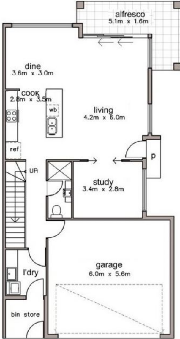
GROUND FLOOR PLAN DWELLING 1
