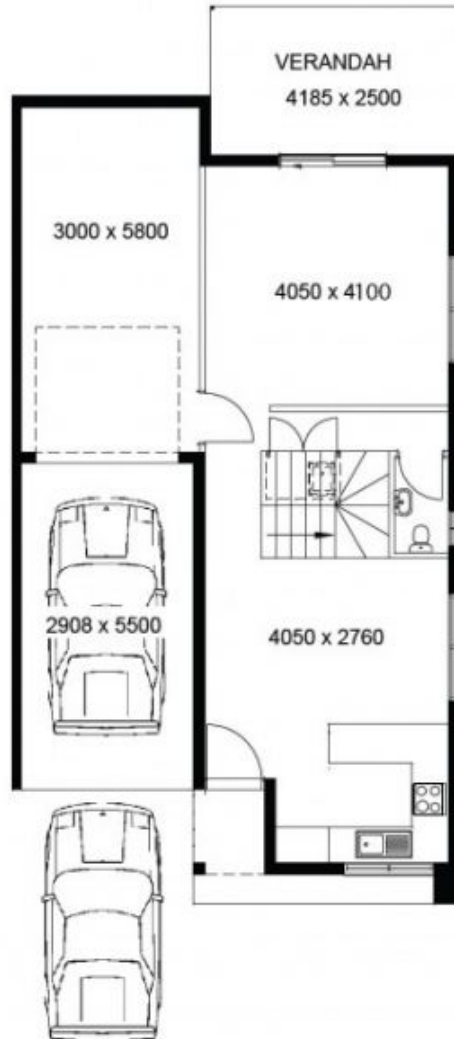
LOT 4 LOWER FLOOR PLAN
