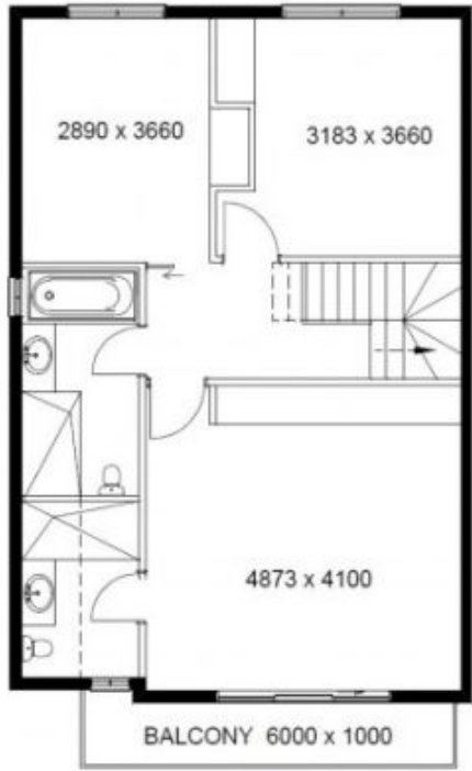
LOT 1 UPPER FLOOR PLAN
