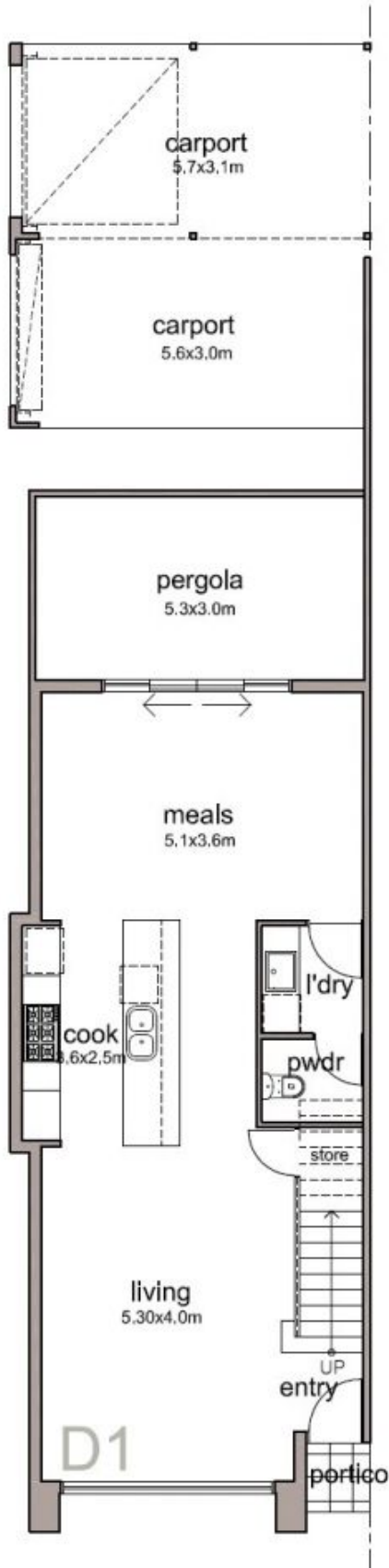
GROUND FLOOR PLAN DWELLING 1
