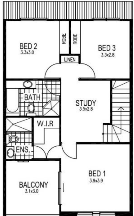
UPPER FLOOR
