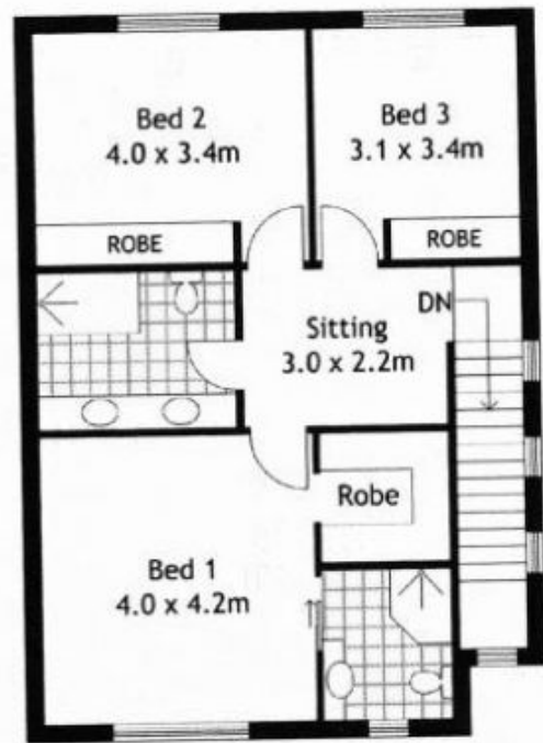
Upper Level Plan
