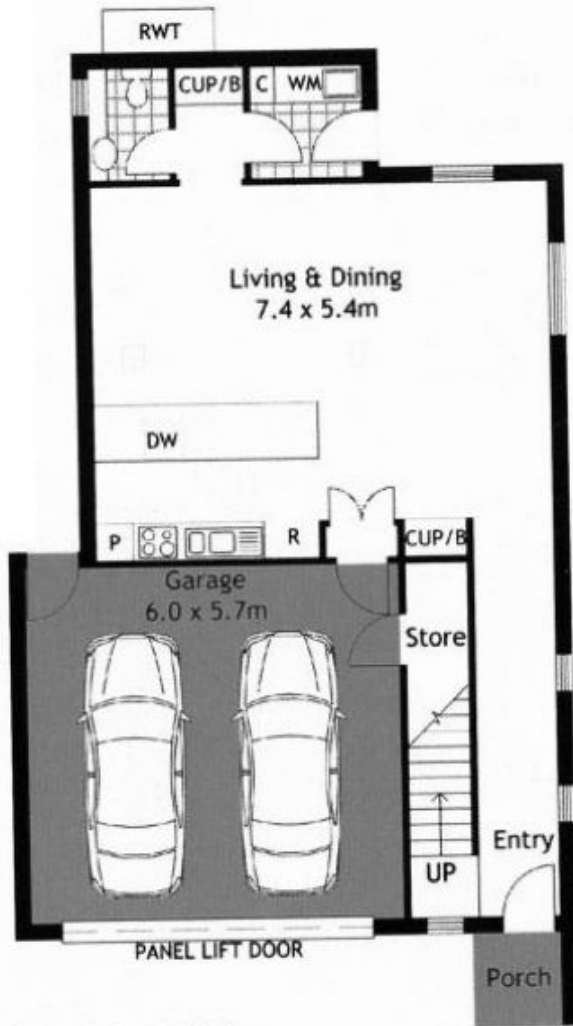
Lower Level Plan
