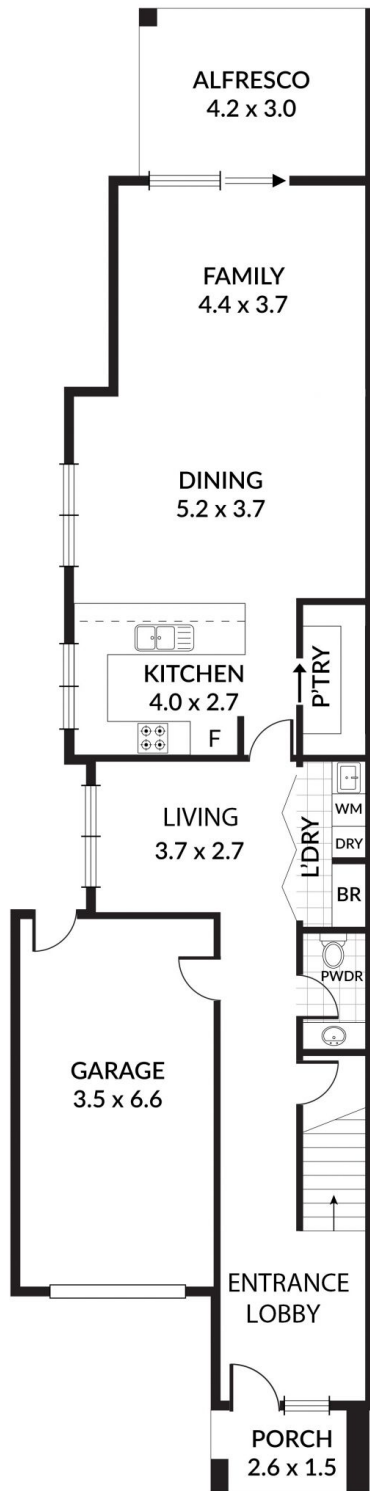
GROUND FLOOR
