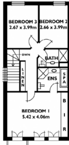
FIRST FLOOR
