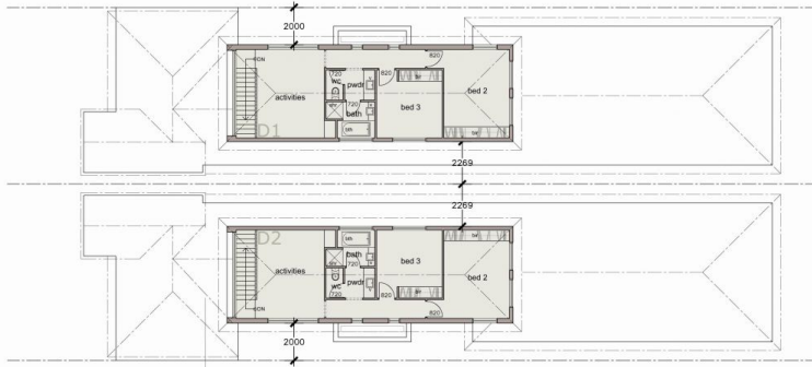
upper floor plan scale 1:100
